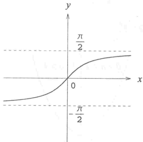
F9*: y = \operatorname{arctg} x
