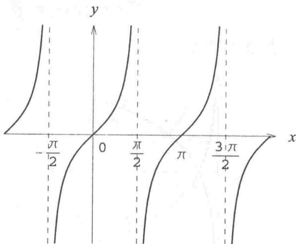
F9: y = \operatorname{tg} x
